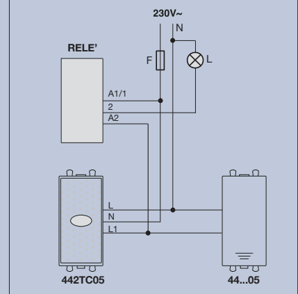
L: carico L: load F: fusibile F 1A H F: fuse F 1A H
